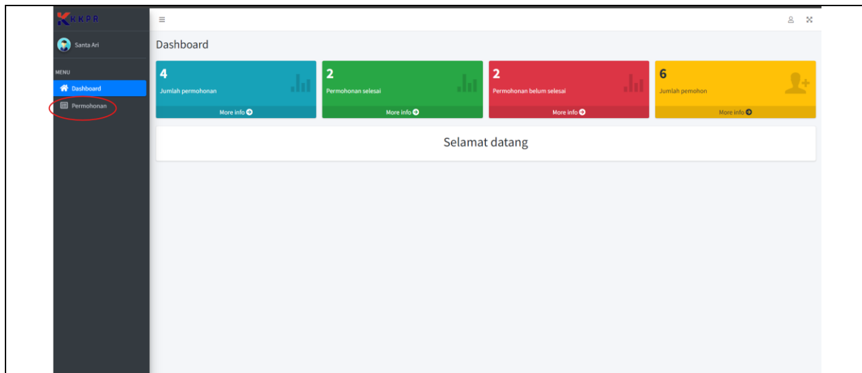
Gambar 3 Halaman Dashboard
